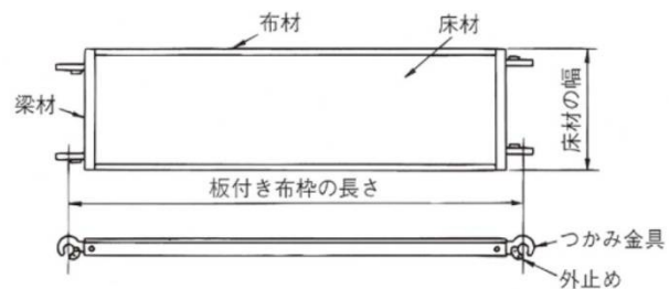
板付き布枠
